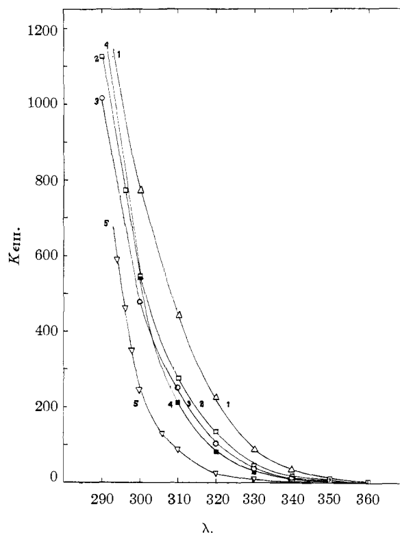
Fig. 2.— K \epsilon_{III} versus \lambda curves: 1, 1-methylpyridinium iodide; 2, 1,2-dimethylpyridinium iodide; 3, 1,4-dimethylpyridinium iodide; 4, 1,2,6-trimethylpyridinium iodide; 5, 1,2,4,6-tetramethylpyridinium iodide.
